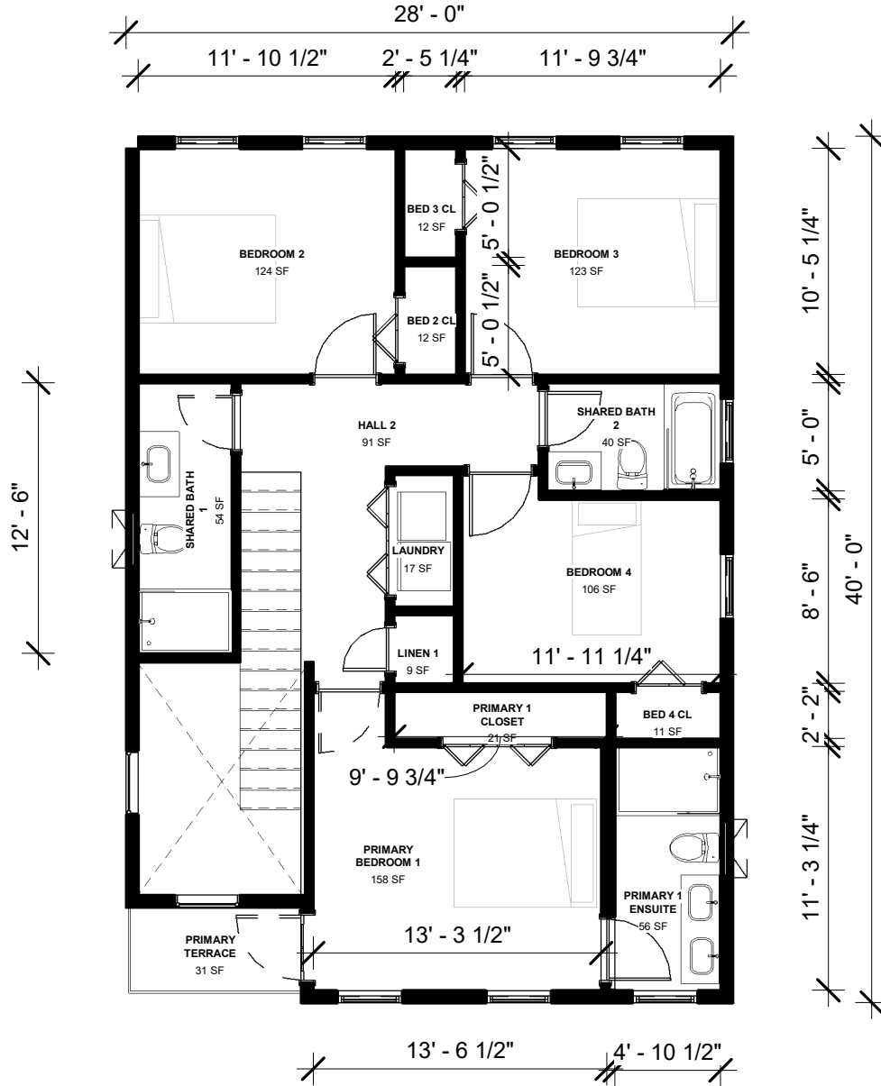
① SECOND FLOOR - MARKETING 1/8" = 1'-0"
