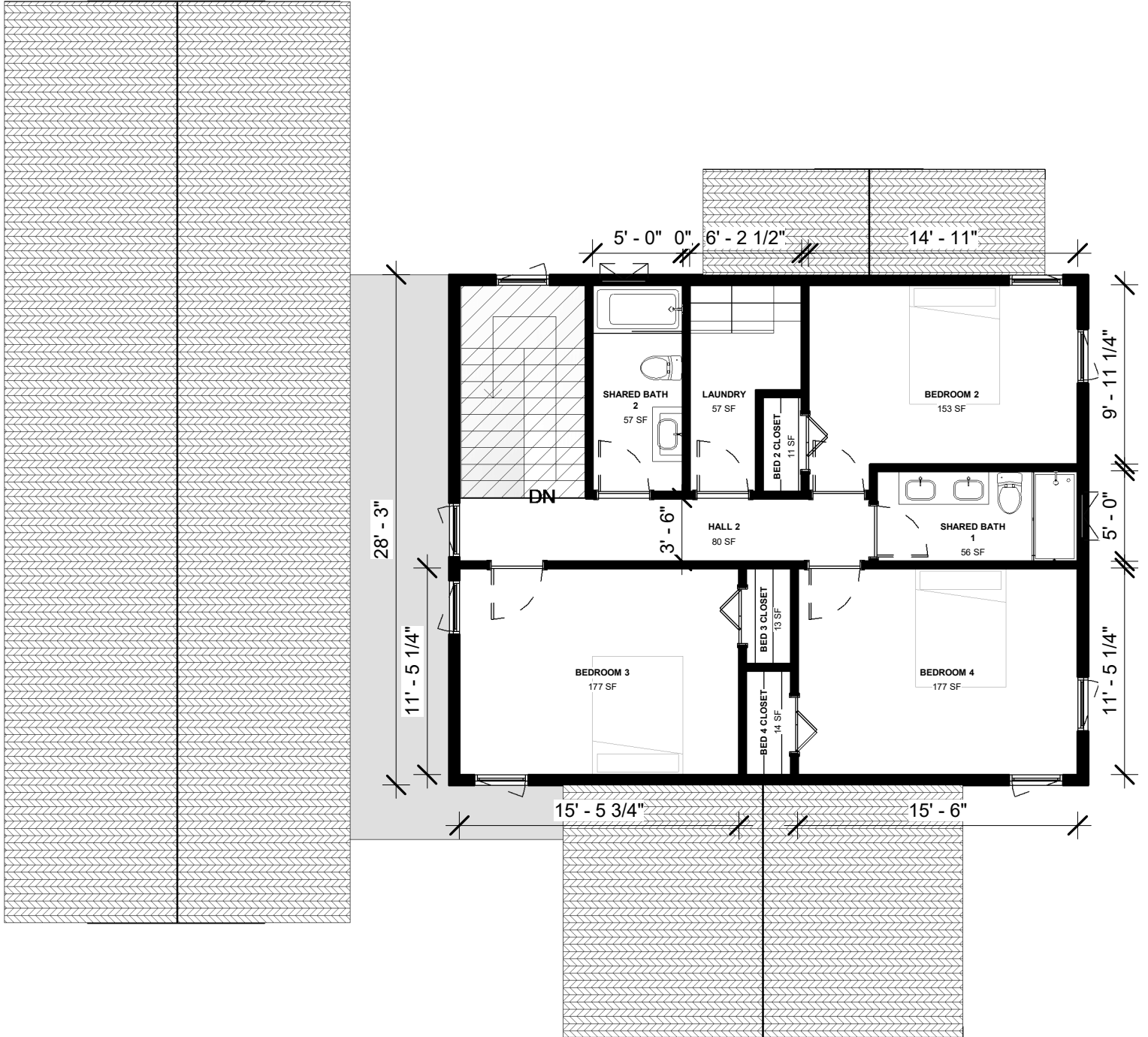
1 SECOND FLOOR - MARKETING PLAN 1/8" = 1'-0"
