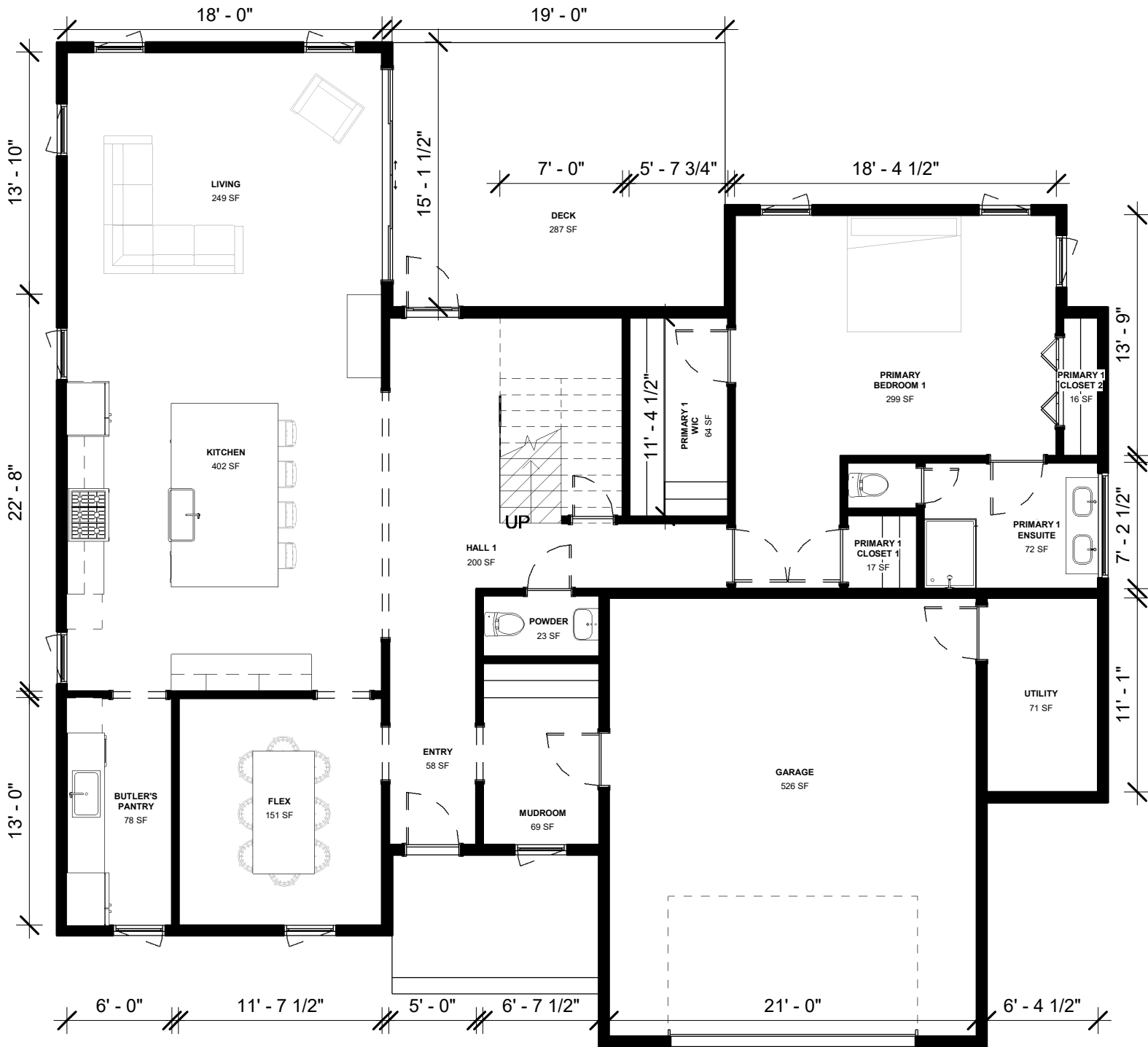
1 FIRST FLOOR - MARKETING PLAN 1/8" = 1'-0"
