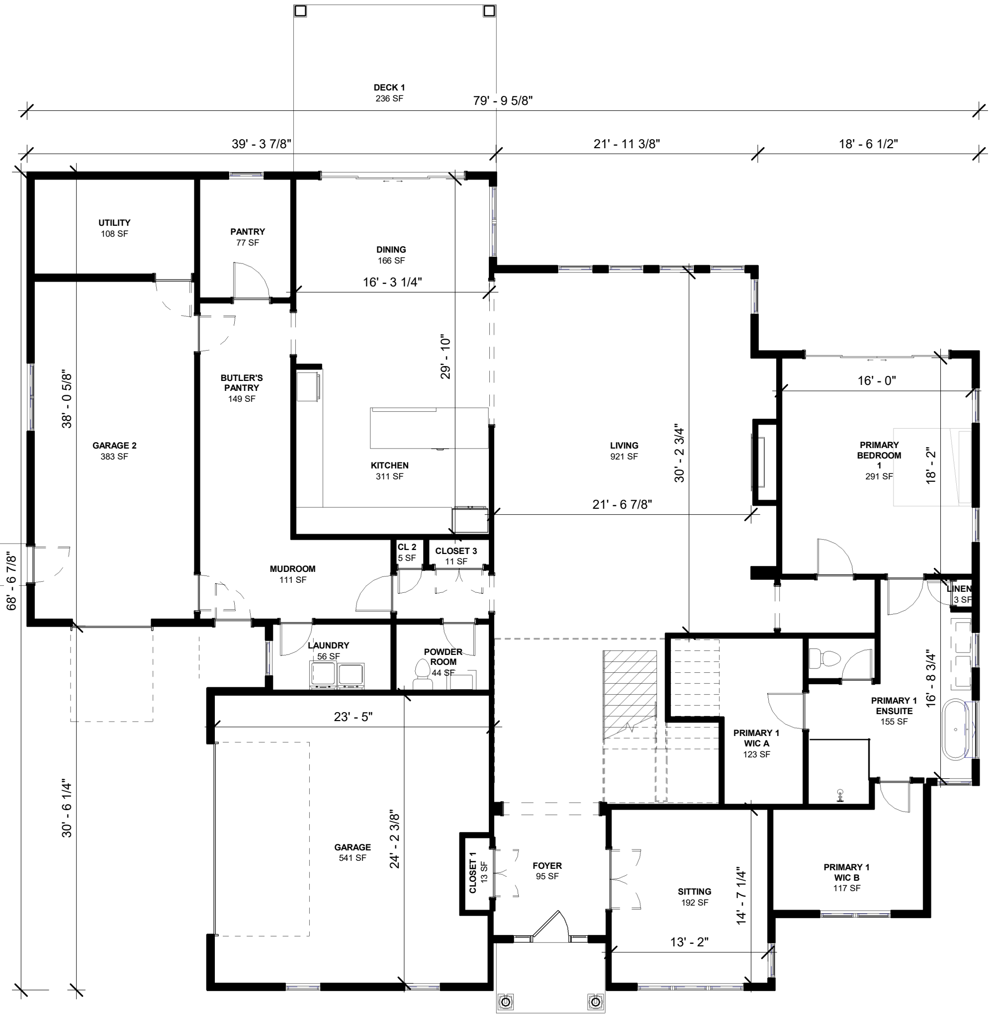
1 FIRST FLOOR MARKETING PLAN 1/8" = 1'-0"
