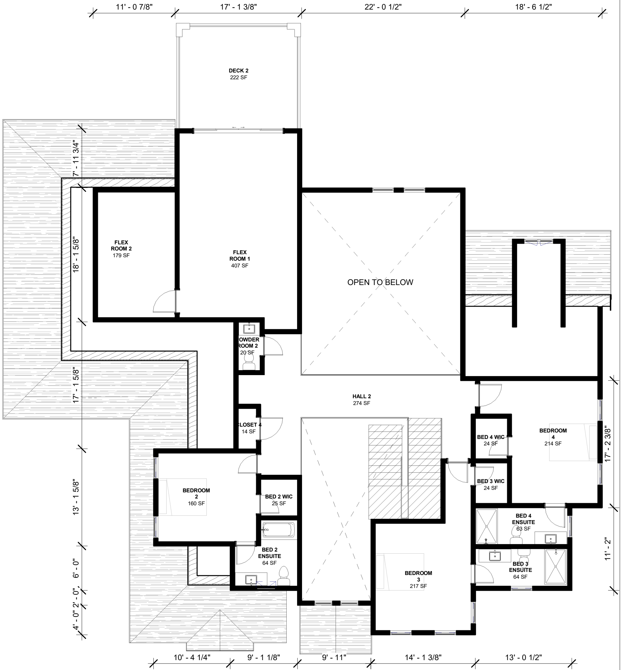
SECOND FLOOR MARKETING PLAN 1/8" = 1'-0"
