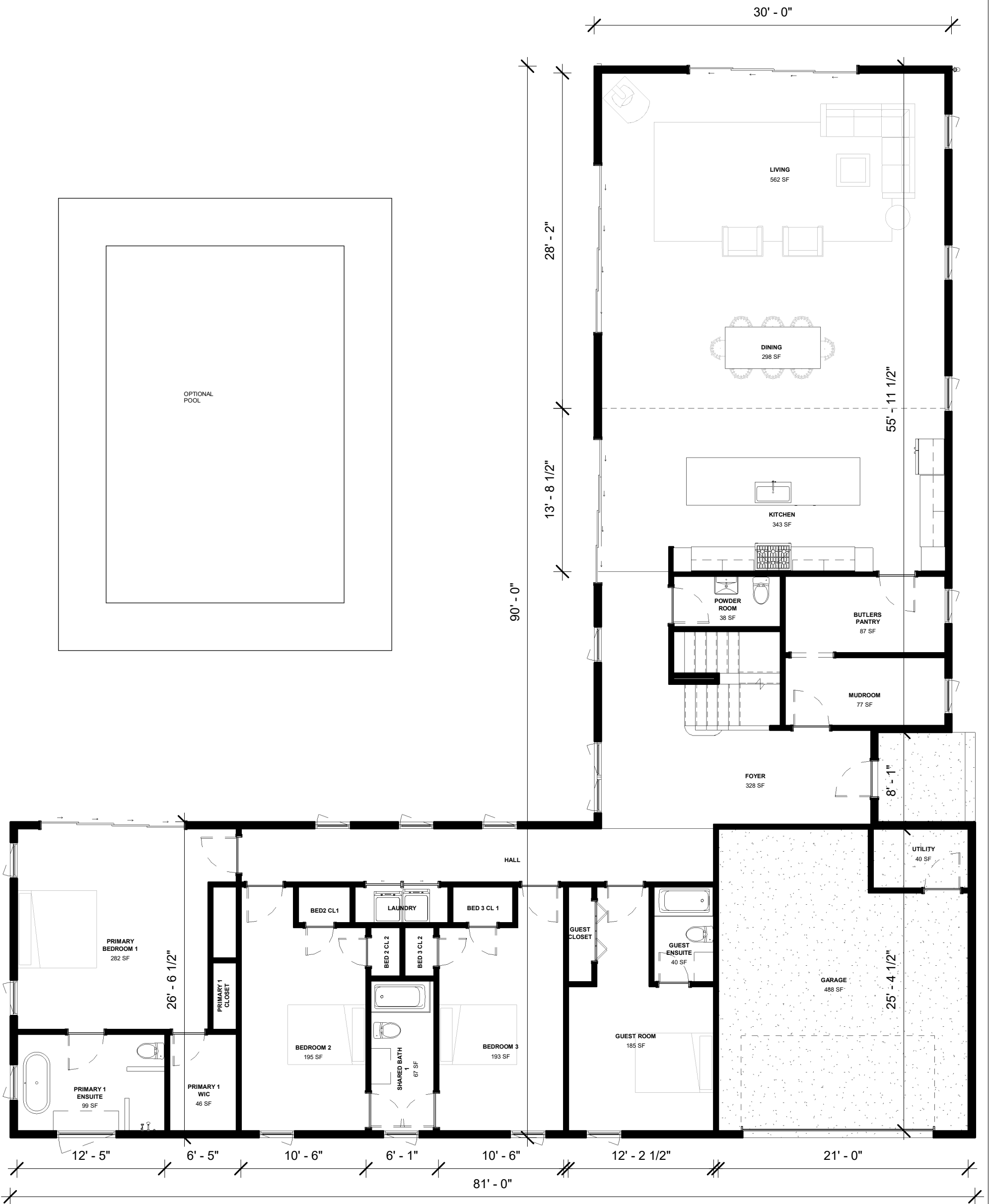
1 FIRST FLOOR MARKETING PLAN 1/8" = 1'-0"
